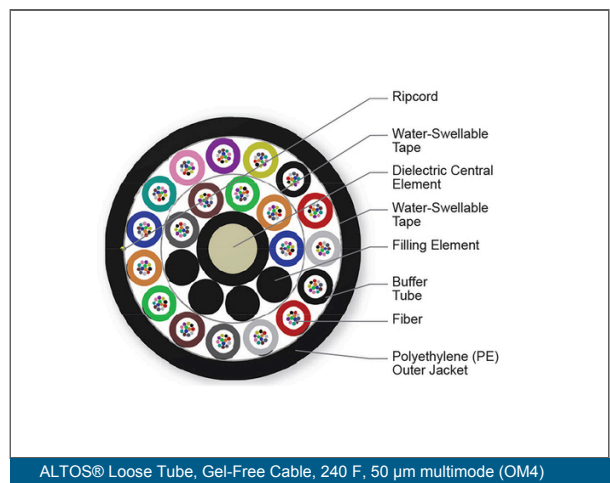
ALTOS® Loose Tube, Gel-Free Cable, 240 F, 50 µm multimode (OM4)
